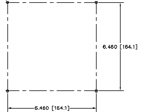
MOUNTING DETAIL
